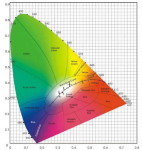
CIE1931
